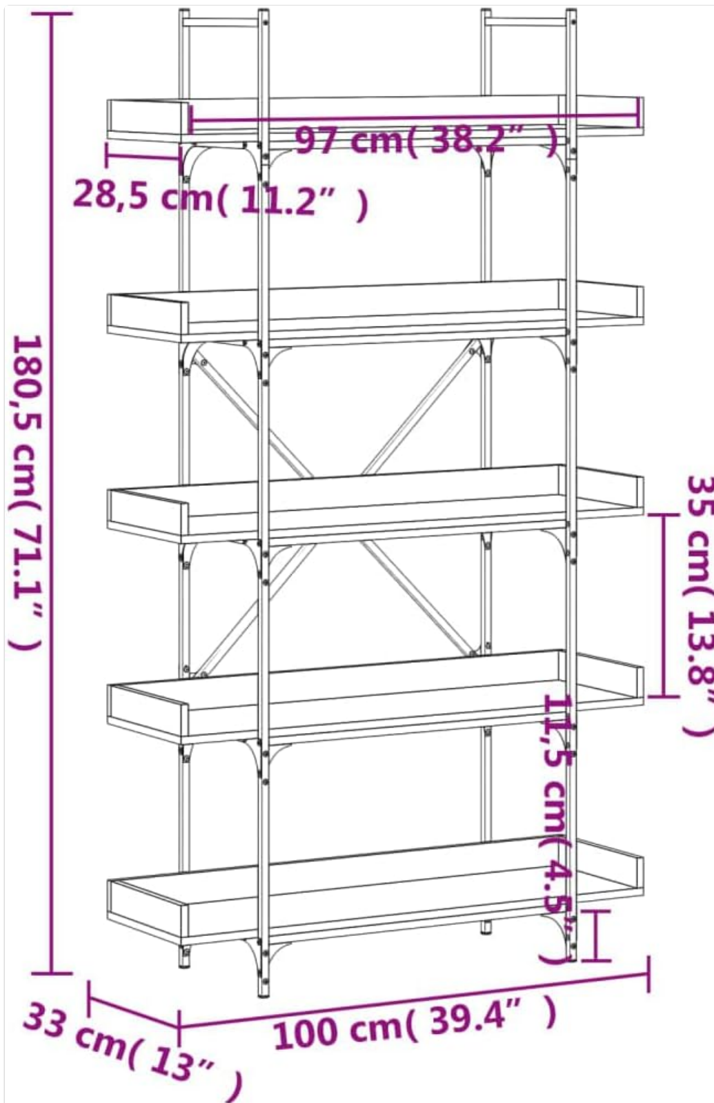
Image: Technical diagram illustrating the precise dimensions of the bookshelf in both centimeters and inches.
