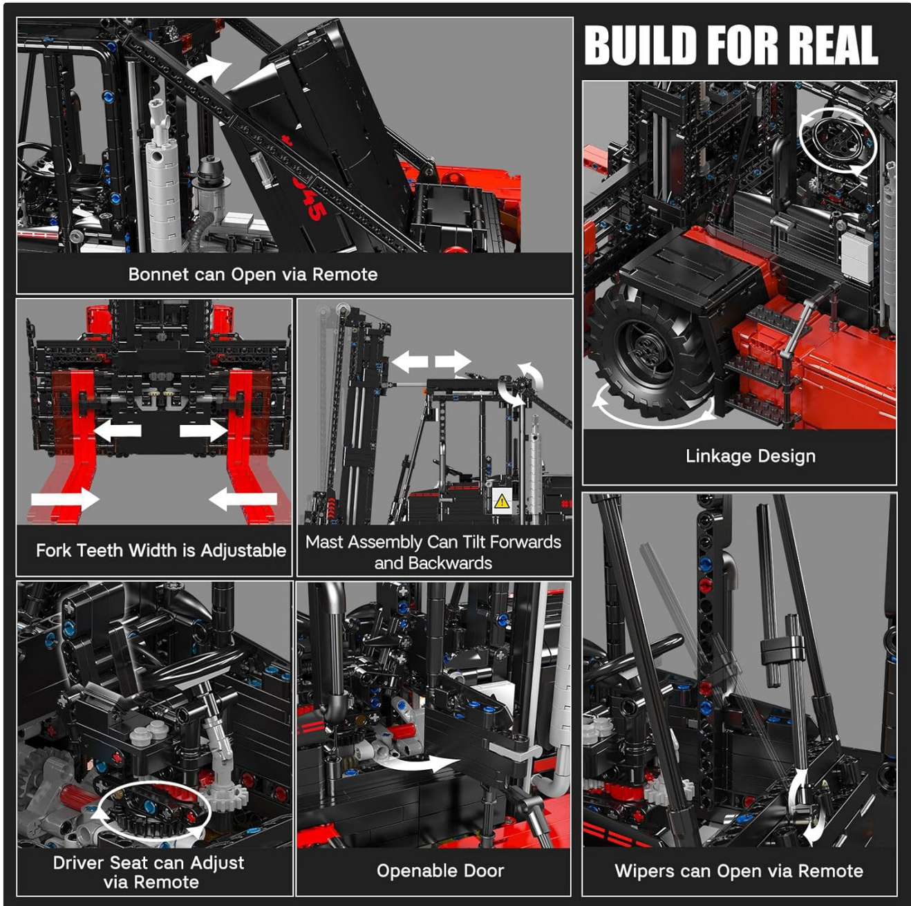
Figure 2: Detailed features of the Mould King 17045 forklift. This image highlights various functional aspects such as the openable bonnet, adjustable fork teeth width, mast tilt mechanism, driver's seat adjustment, openable door, and functional wipers, all built from the blocks.
