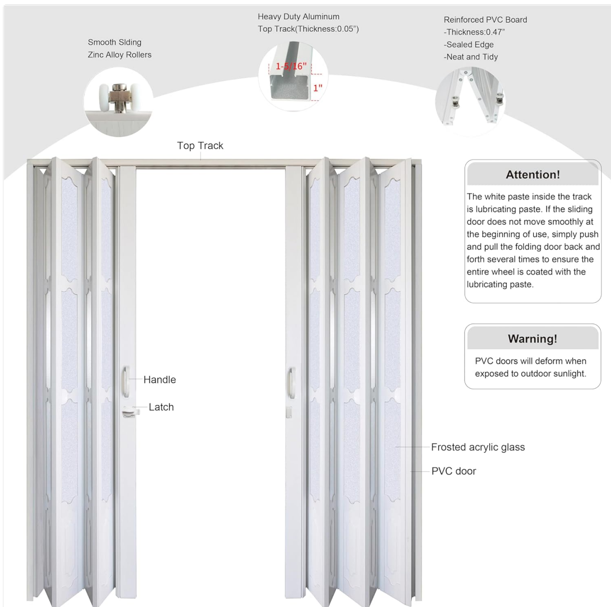
Figure 5: Important notes regarding the lubricating paste in the track and a warning about PVC door deformation when exposed to outdoor sunlight.
