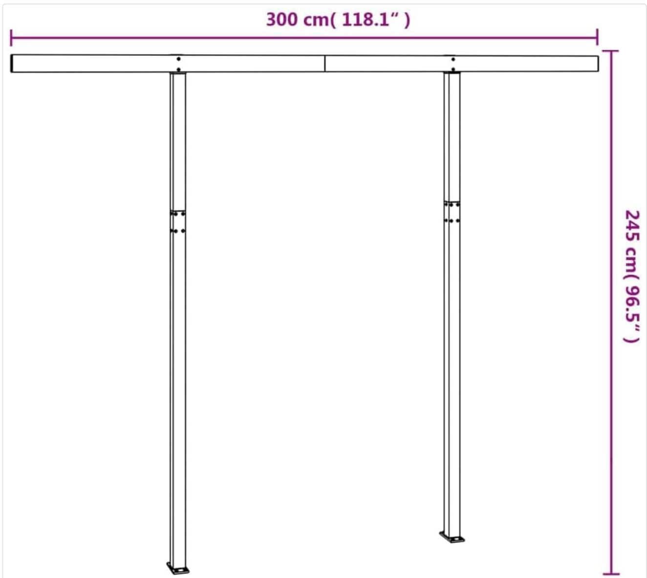
Image 3: Dimensional diagram of the awning post set, showing width and height.
