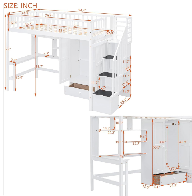
Image 4.1: Detailed dimensions of the Polibi Twin Loft Bed, including length, width, height, and internal measurements for the desk, wardrobe, and staircase.
