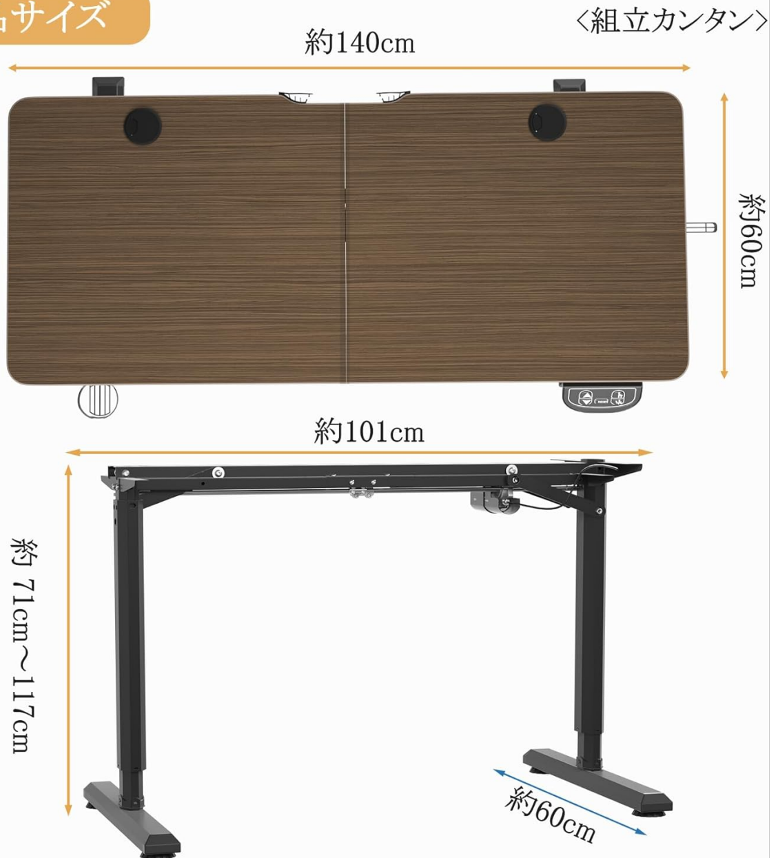
Image: Overhead view showing the two-piece tabletop and frame dimensions (approx. 140cm width, 60cm depth, height adjustable from 71cm to 117cm).
