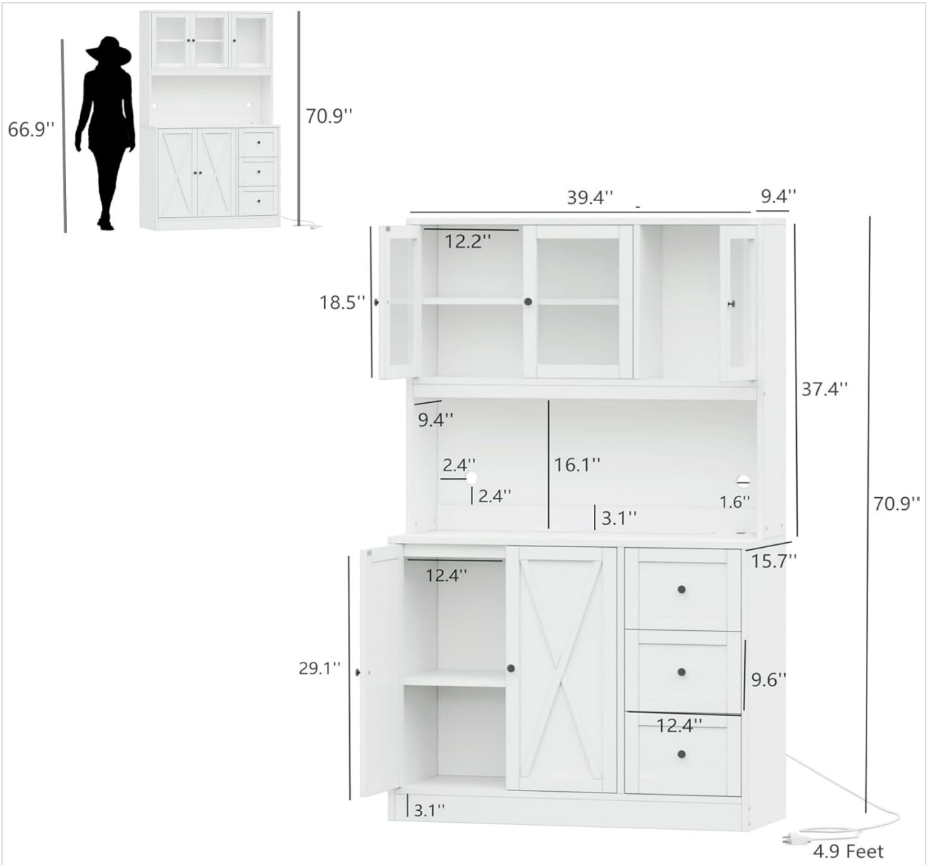
Figure 7.1: Detailed dimensions of the Irontar CWG011E Kitchen Pantry.
