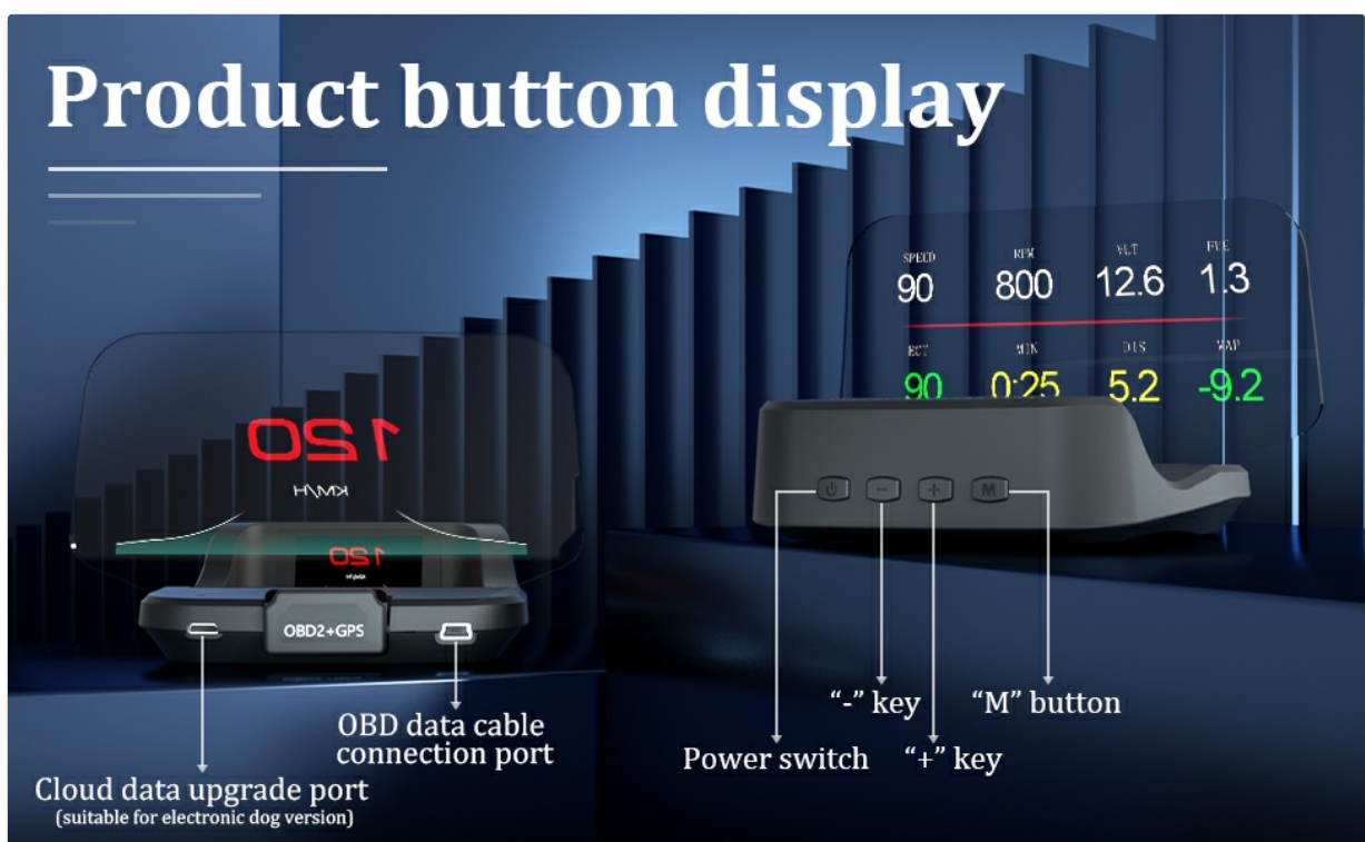
Figure 6: The C2 HUD supports two power cords: OBD cable for dual system and cigarette lighter for GPS only.
