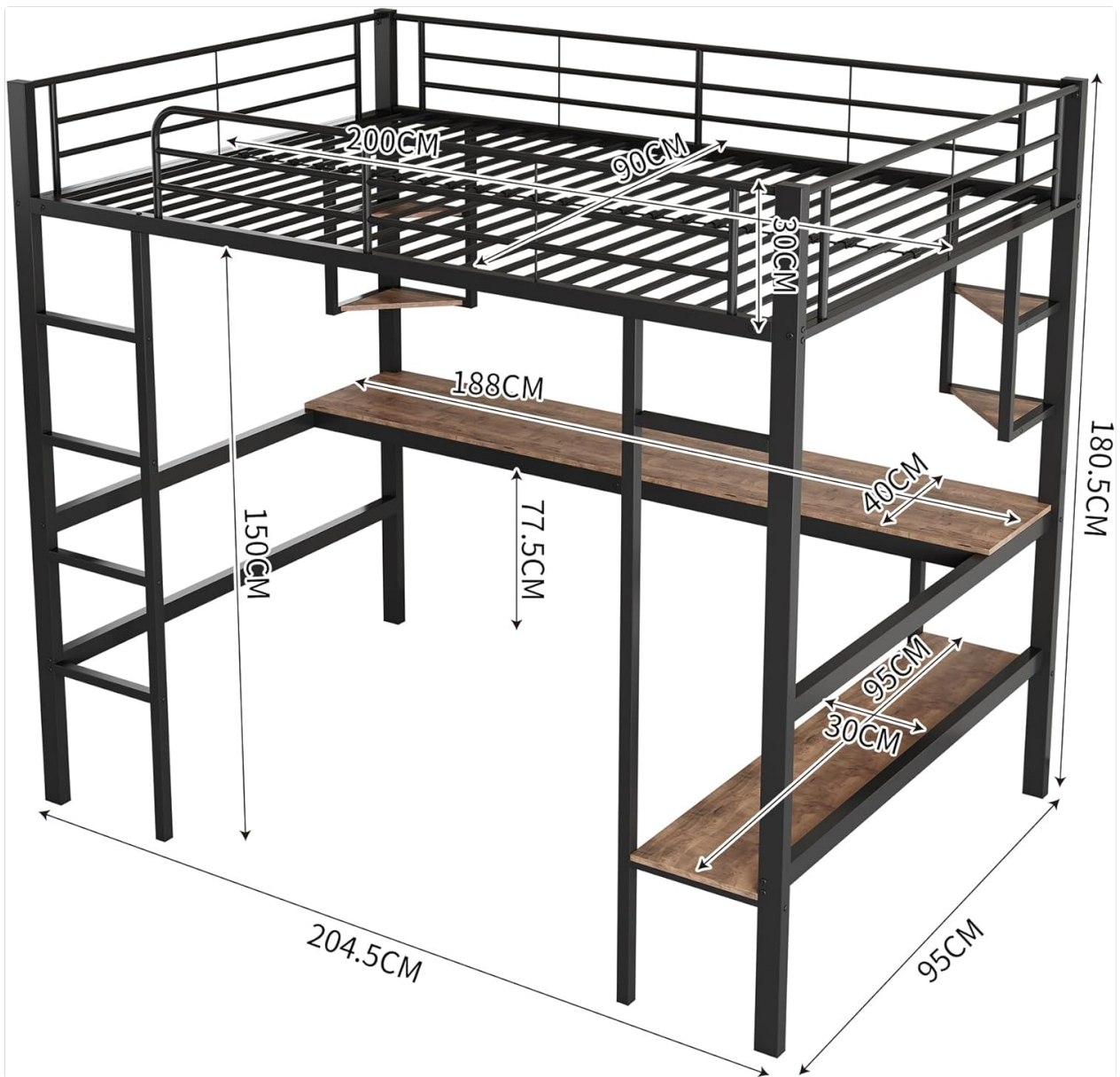
Figure 1: Dimensional diagram of the Moimhear Loft Bed. This image illustrates the overall dimensions and key measurements of the assembled bed, including the height, length, width, and desk/shelf dimensions, which are crucial for assembly and placement.
