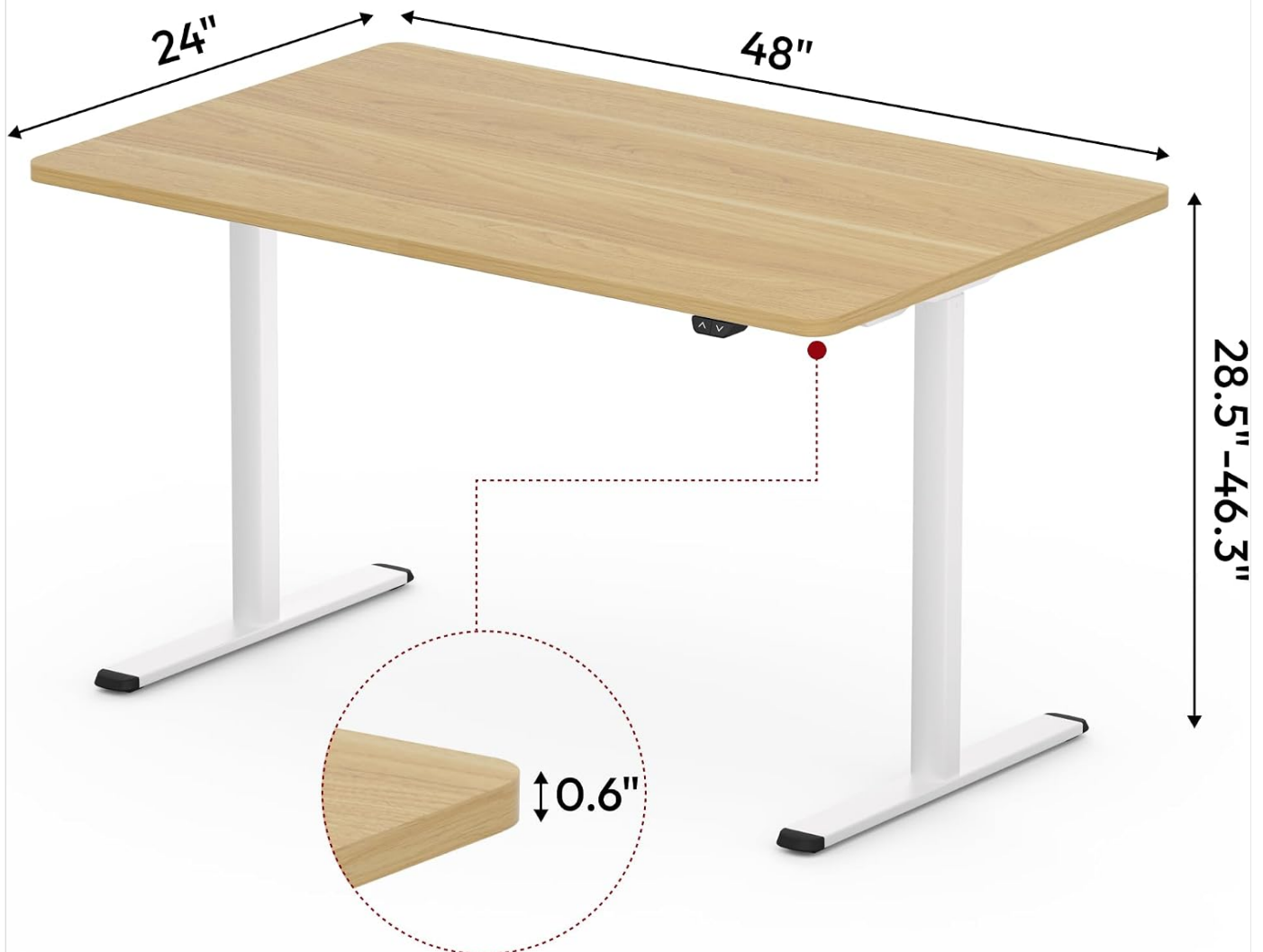
Image: Diagram showing the dimensions of the SANODESK Standing Desk, including a desktop size of 48" x 24", a thickness of 0.6", and an adjustable height range of 28.5" to 46.3". It also indicates a weight capacity of up to 110 lbs.
