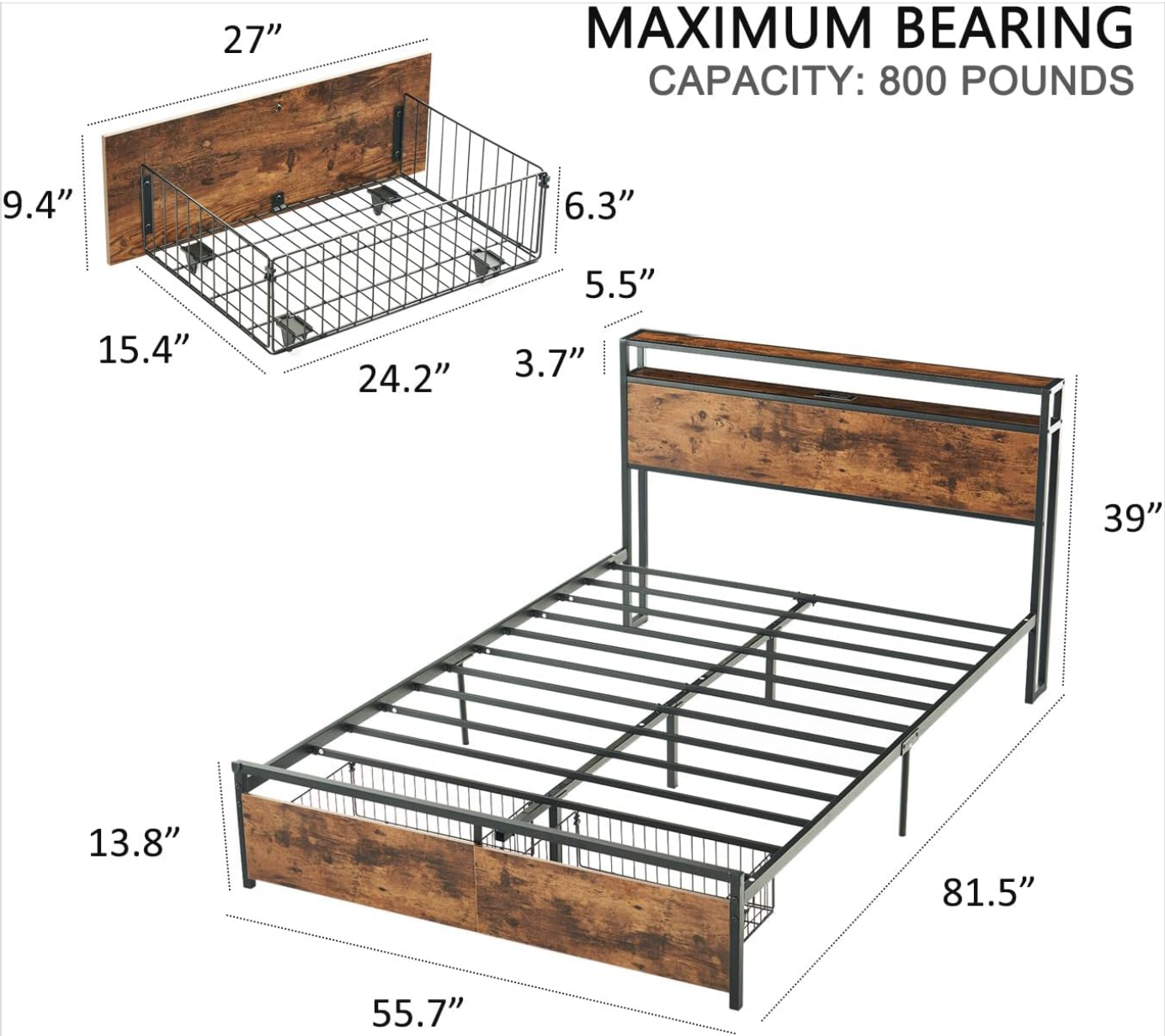
Image: Detailed dimensions of the bed frame and storage components, indicating a maximum bearing capacity of 800 pounds.
