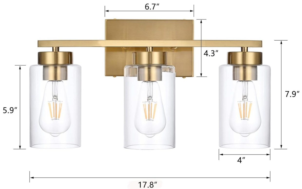
Detailed dimensions of the A1A9 3-Light Vanity Light fixture, showing height, length, and width.
