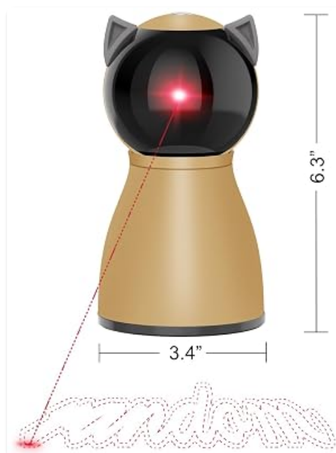
Image: Diagram illustrating the manual vertical adjustment (50°) and automatic horizontal swing (60°) of the laser head.
