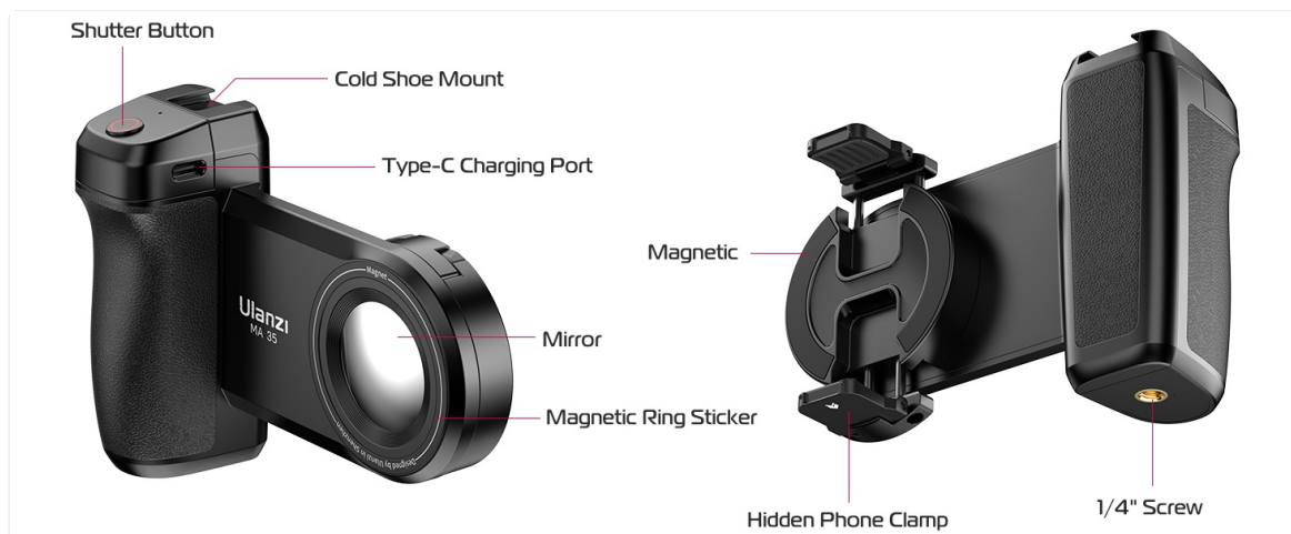
Figure 1: Key components of the ULANZI MA35 Phone Camera Grip.
