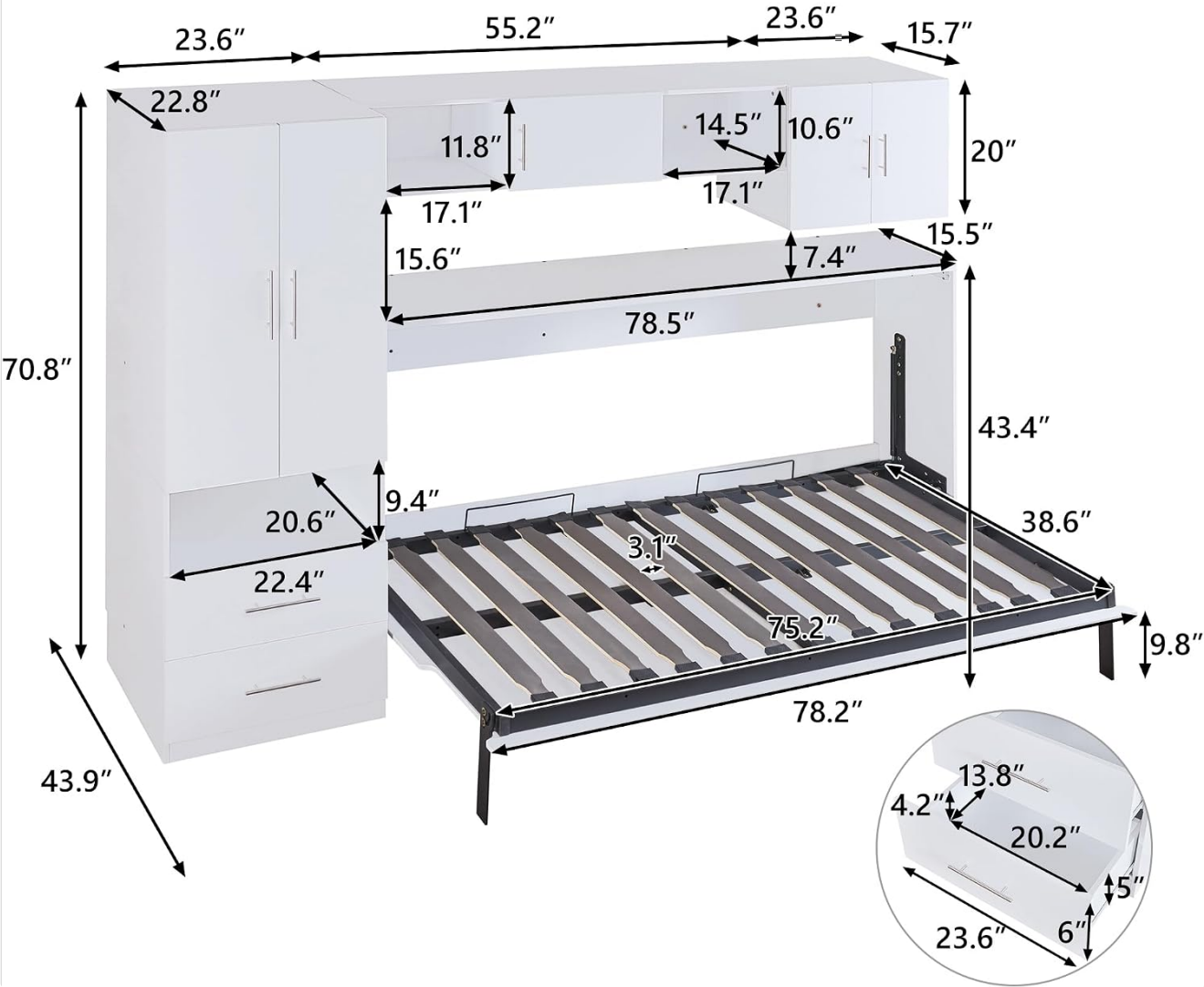
Image: Detailed dimensional drawing of the SOFTSEA Murphy Bed, showing overall length, width, height, and internal measurements of storage components and bed frame.
