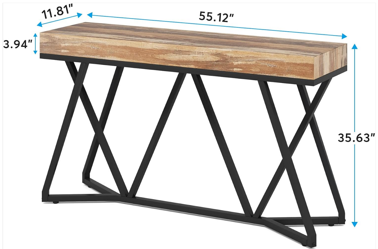
Image: Dimensional diagram illustrating the width, depth, height, and tabletop thickness of the console table.
