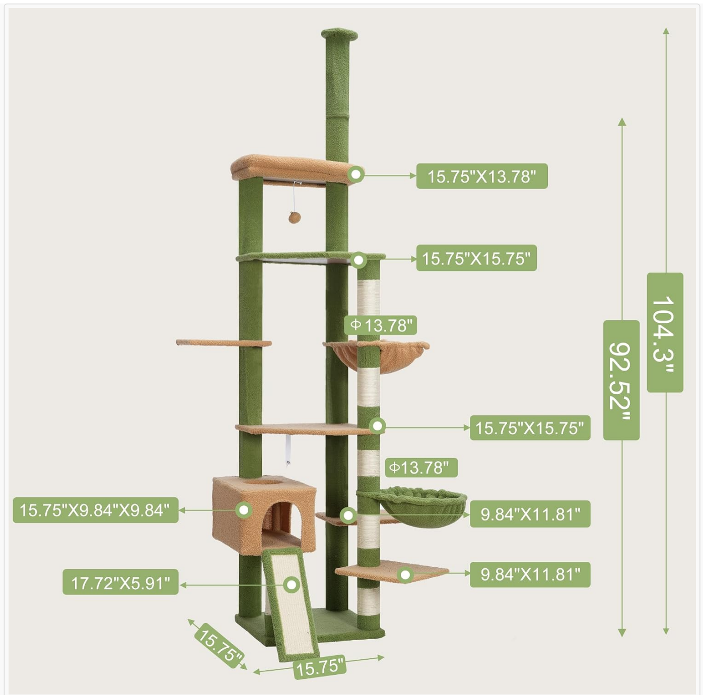
Figure 8.1: Dimensional overview of the Heybly Cat Tree HCT091GM.
