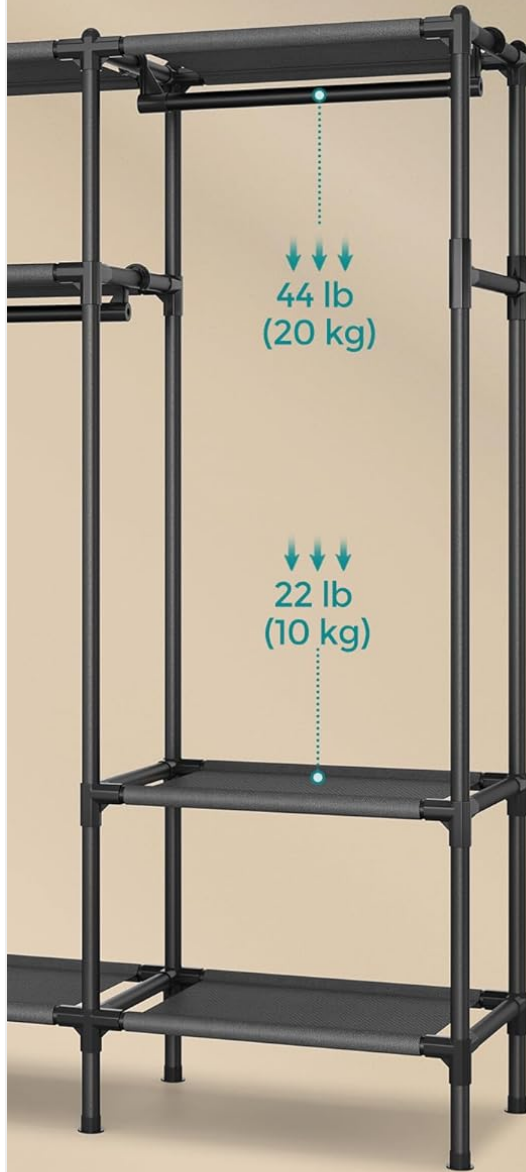
Image 5.2: Details on the robust construction, including thick steel tubes, quality non-woven fabric, and reinforced plastic connectors, along with load capacities.
