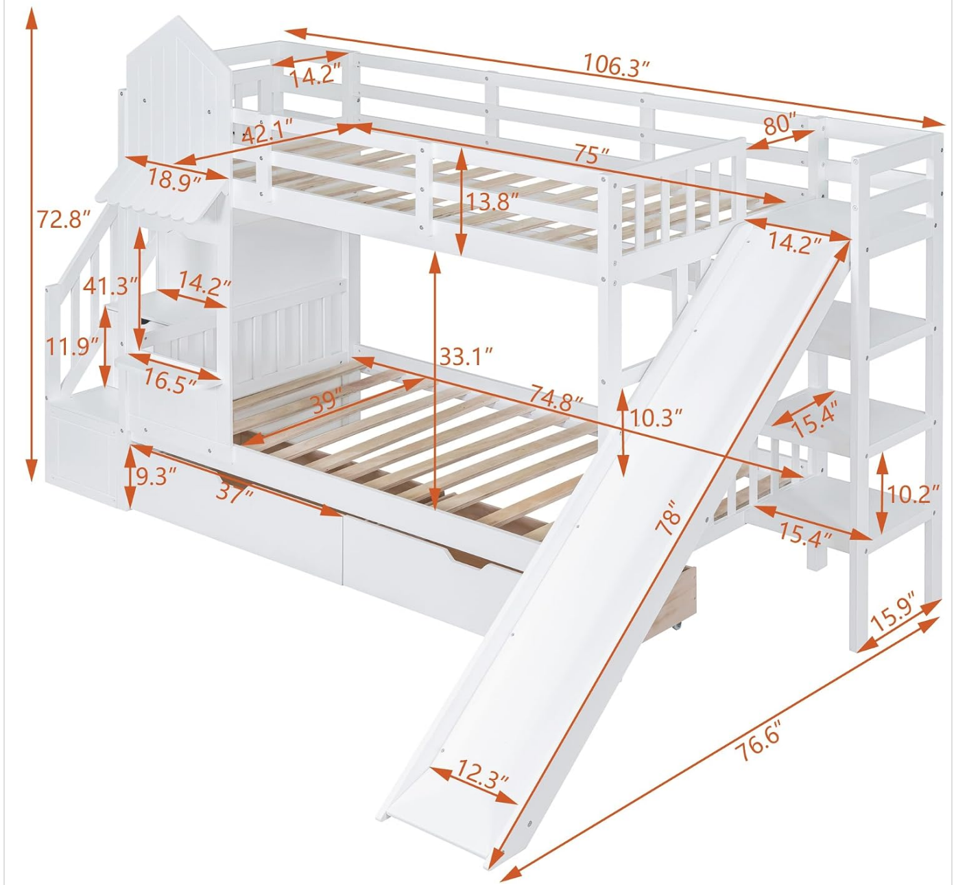
Figure 4: Dimensional drawing of the bunk bed, providing overall and detailed measurements for planning and assembly.
