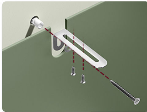
Image: A diagram illustrating the proper installation of the anti-tip kit, showing the bracket attached to the cabinet and secured to the wall.
