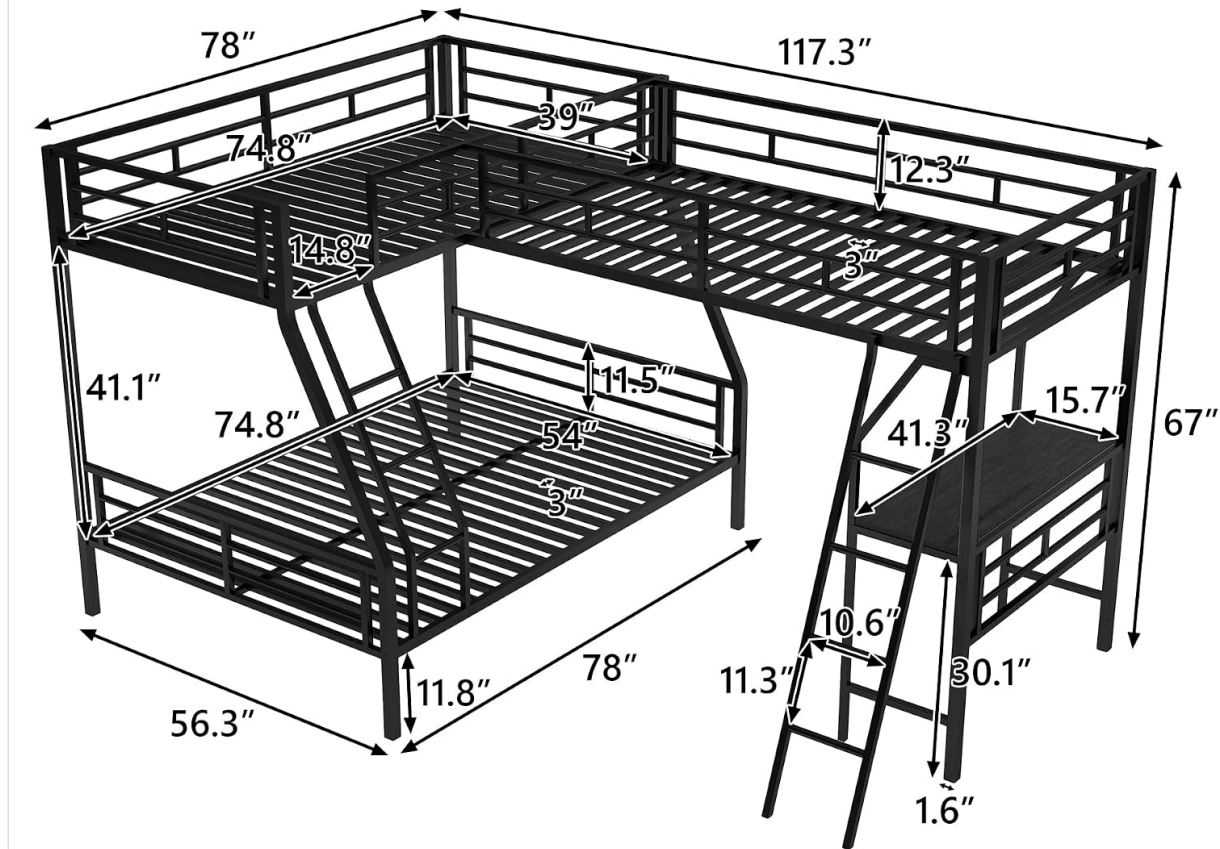
Image 3.1: Detailed dimensions of the bunk bed for assembly planning.
