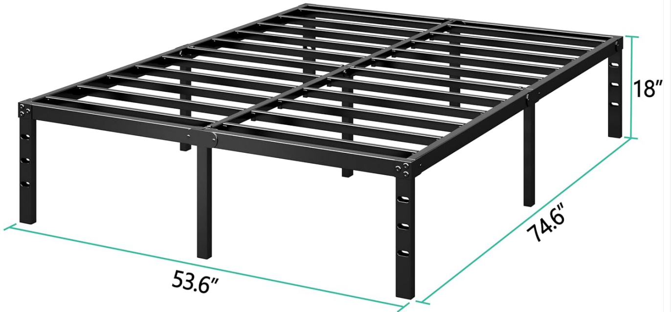
Figure 4.2: Diagram illustrating the full size bed frame dimensions (74.6"L x 53.6"W x 18"H for the 18-inch variant, similar for 16-inch).
