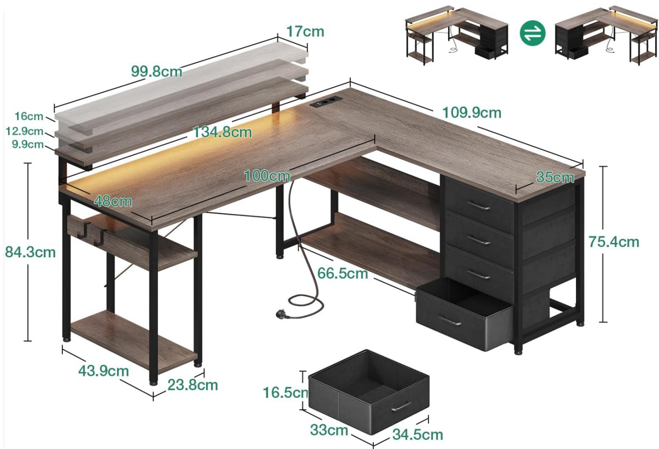
Image: Desk dimensions and illustration of the reversible L-shaped configuration.
