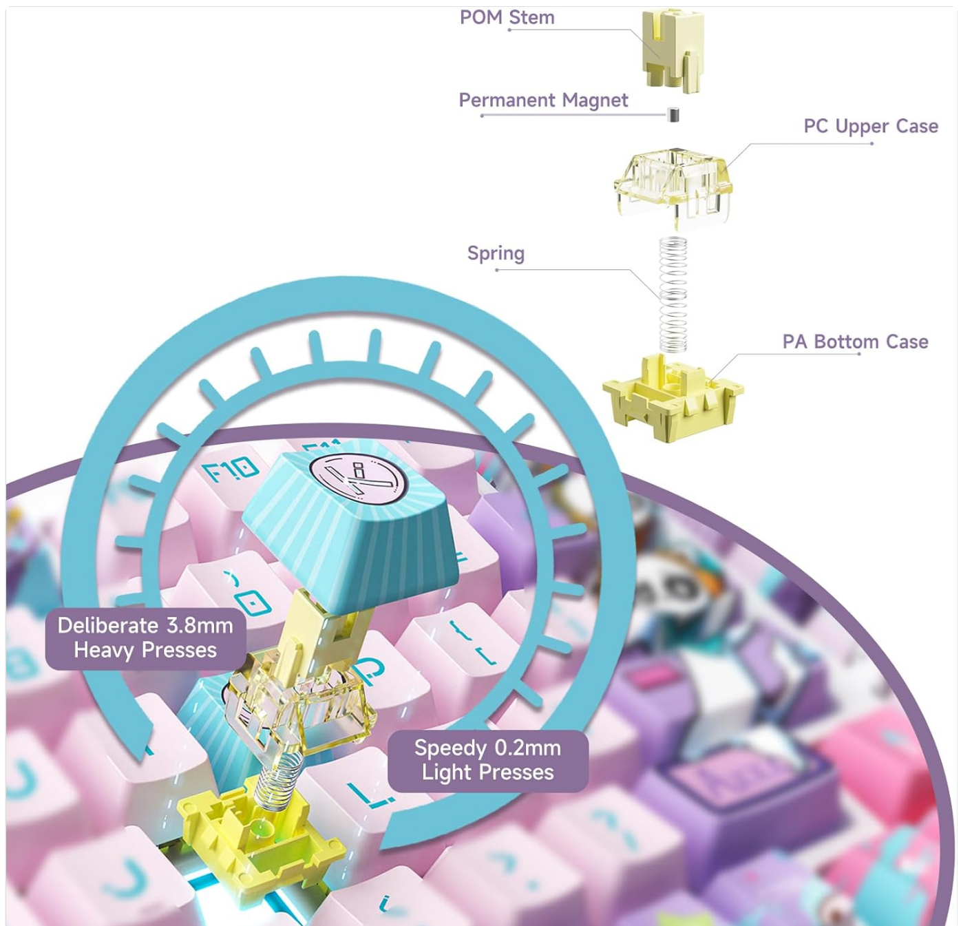
Figure 4: Magnetic Switch Components.
