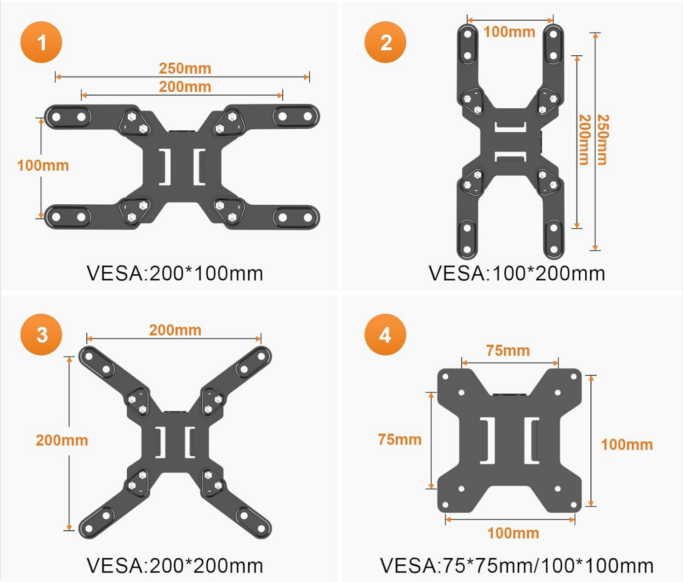
Image: Detailed diagrams illustrating various VESA mounting patterns supported by the mount, including 75x75mm, 100x100mm, 100x200mm, 200x100mm, and 200x200mm.
