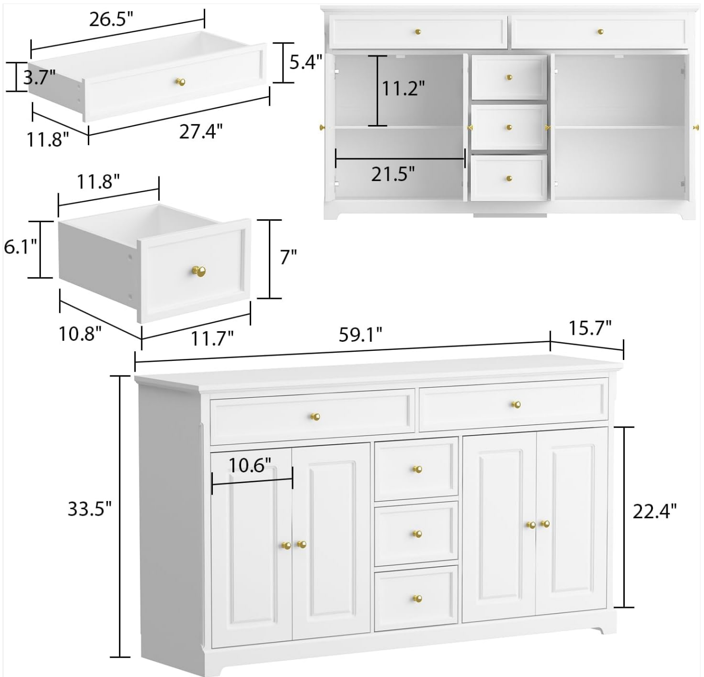
Image 3.1: Dimensional diagram of the buffet cabinet, including overall dimensions and internal compartment measurements, useful for planning placement and understanding component sizes during assembly.
