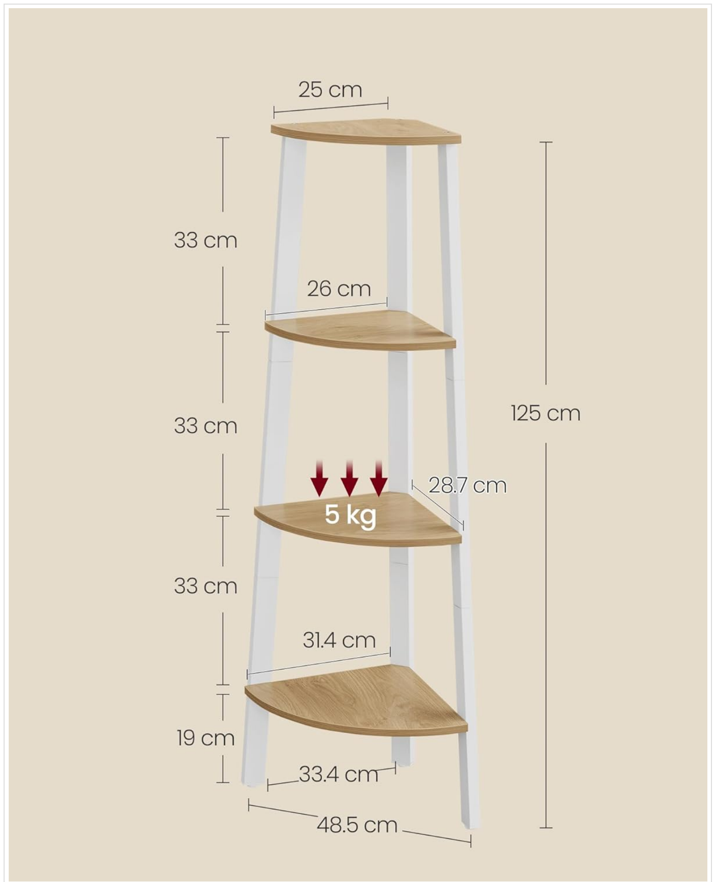
Image 2.1: Detailed dimensions of the 4-tier corner shelf, including shelf spacing and overall height. Maximum load per shelf is 5 kg.
