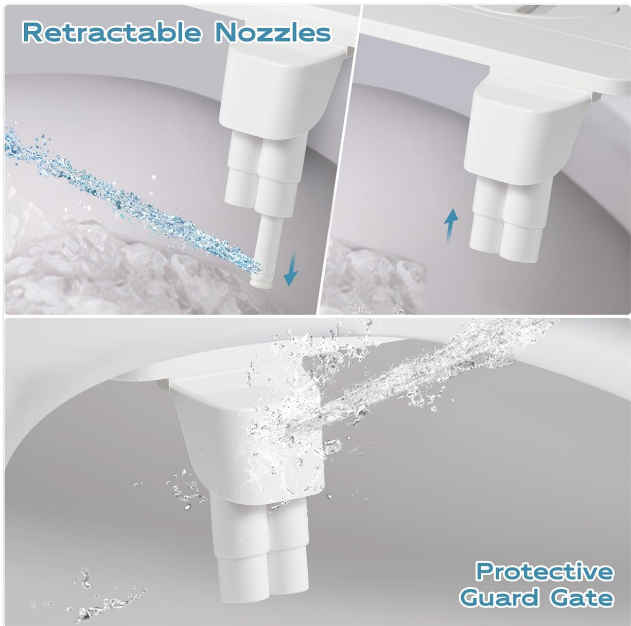
Image: Retractable nozzles and protective guard gate mechanism.
