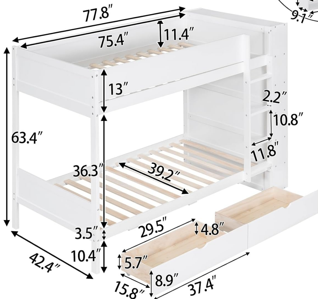
Image: A technical diagram showing all key dimensions of the bunk bed in inches, including overall length, width, height, and internal measurements for bunks and storage.
