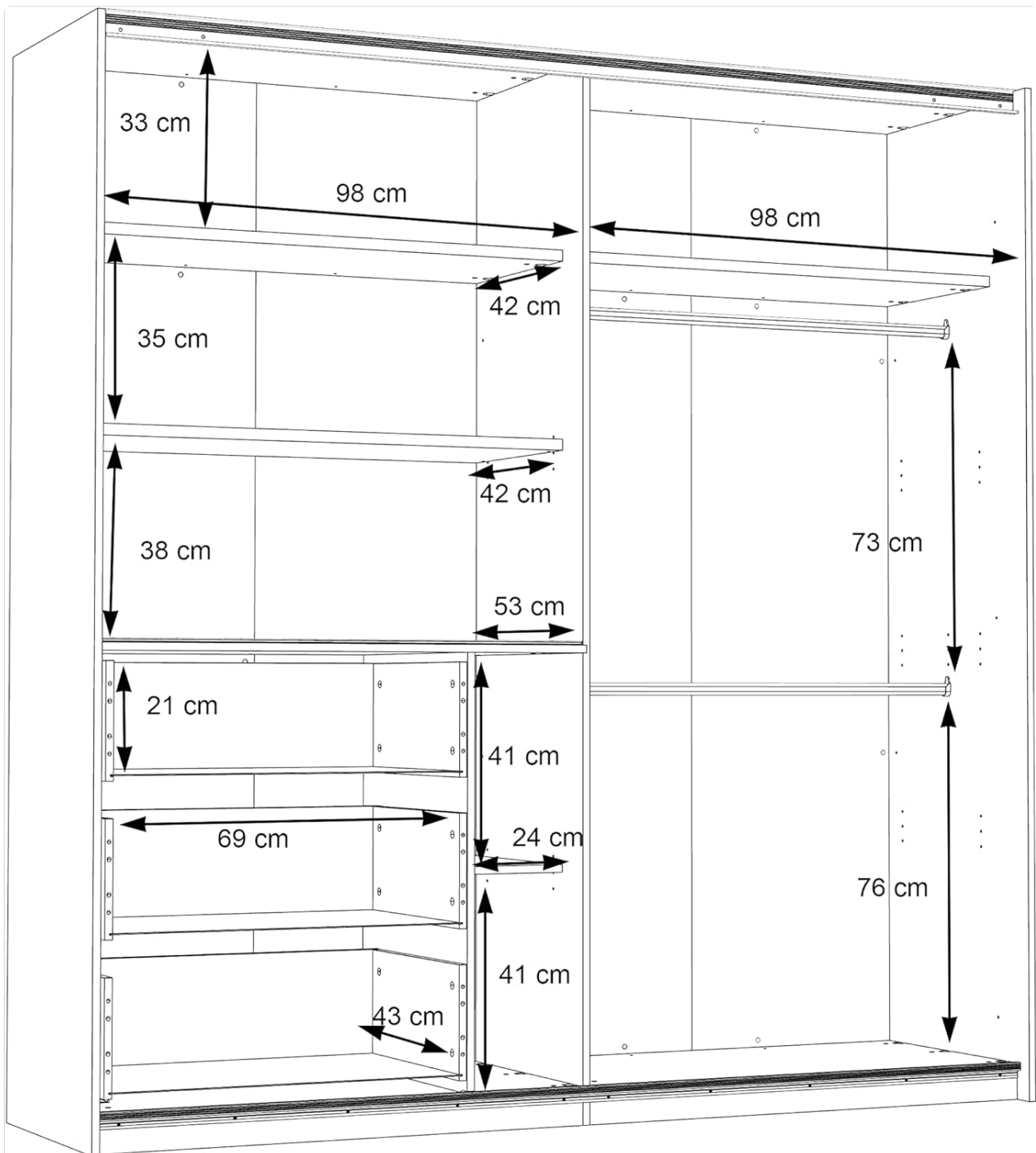
Image 8.2: Internal layout and dimensions diagram.
