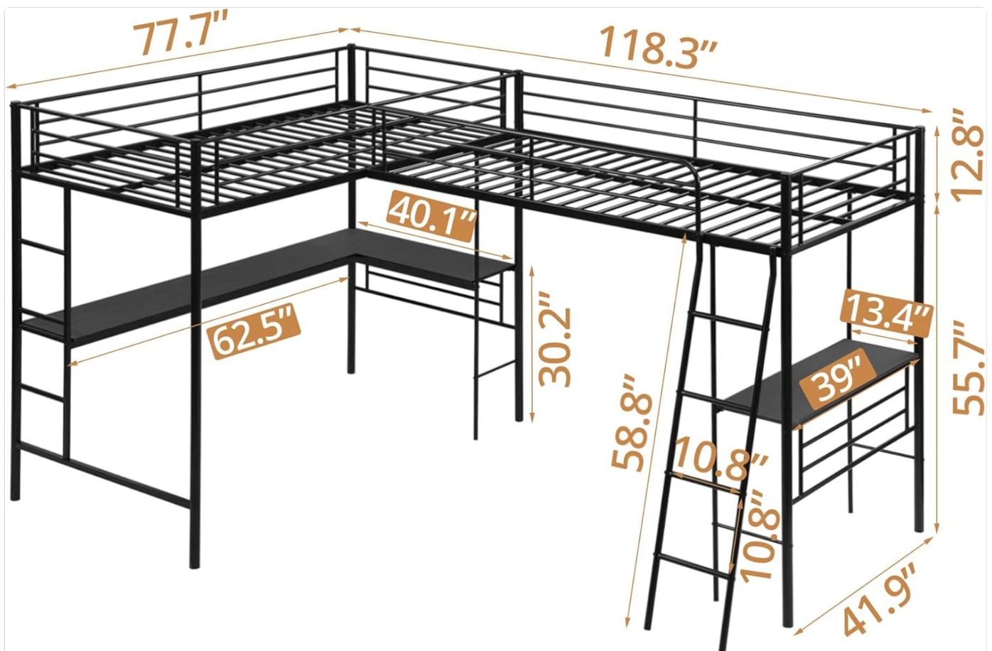
Figure 2: Detailed dimensions of the L-shaped loft bed, showing length, width, and height measurements for proper space planning.
