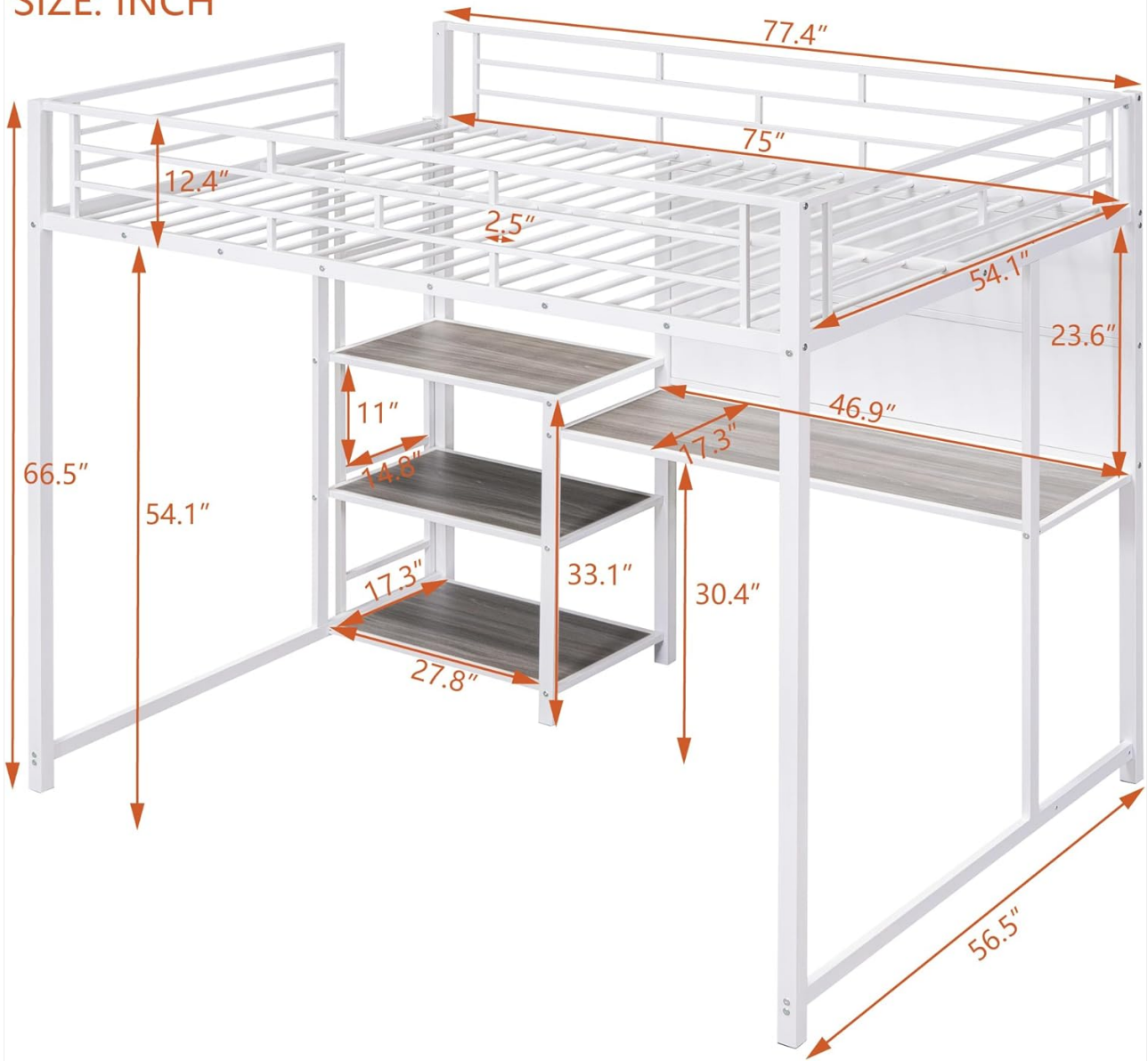
Detailed dimensions of the Bellemave Full Size Metal Loft Bed, showing overall length, width, height, and specific measurements for the desk, shelves, and under-bed clearance.
