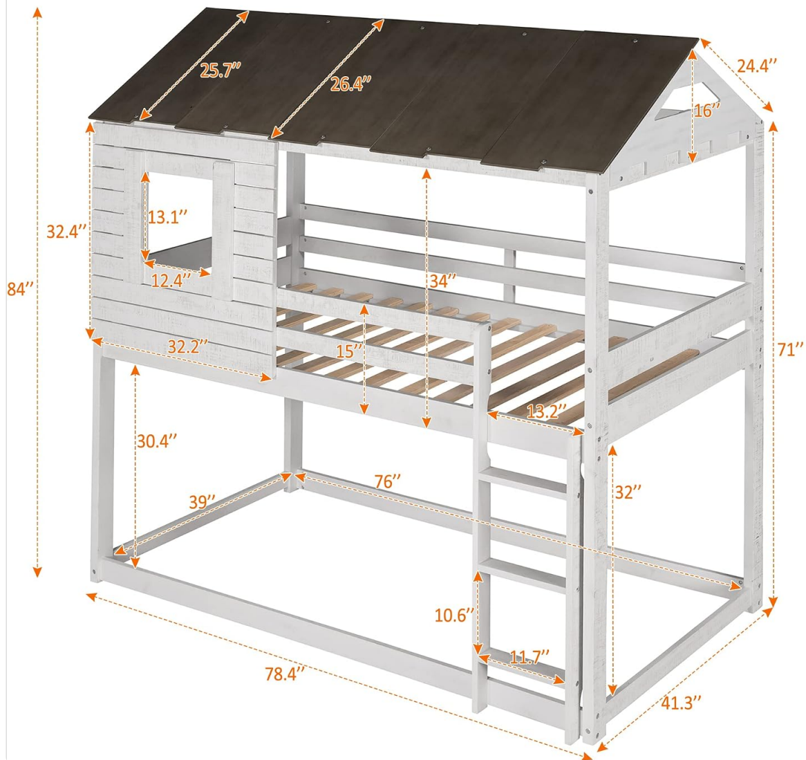
Figure 2: Overall dimensions and key measurements of the bunk bed structure.
