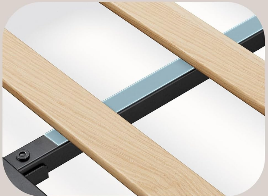
Figure 3: Solid Wood Slats with Velcro and Mute Bars Design
