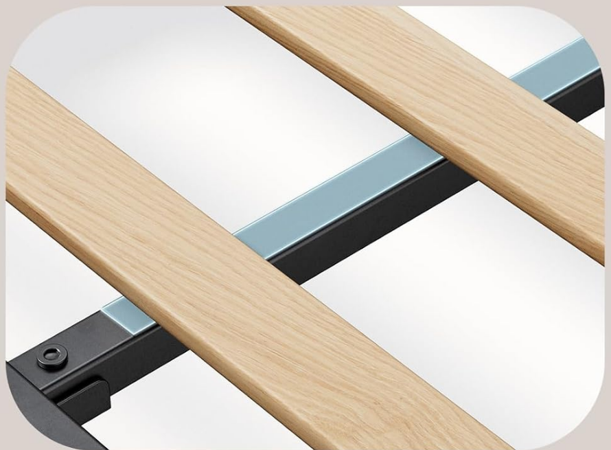
Figure 3: Detail of solid wood slats with Velcro fastening and mute bars for noise reduction.
