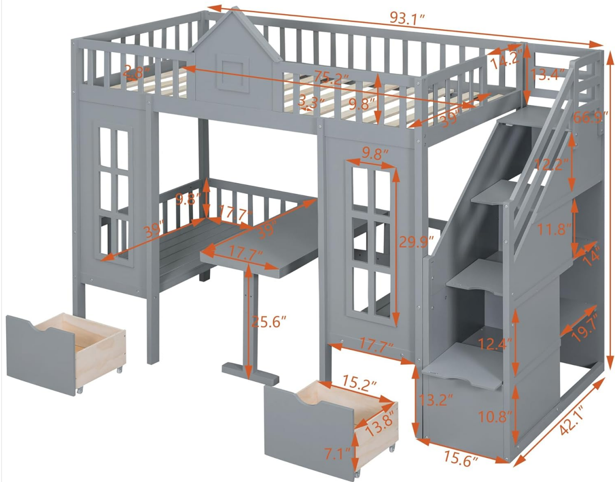
Image 8.1: Detailed dimensions of the Polibi Twin-Over-Twin Bunk Bed.
