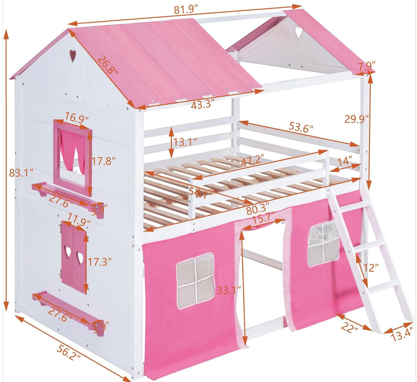
Figure 2: Detailed dimensions of the Aiuyesuo Full Size House Bed. Refer to this diagram for precise measurements during assembly and placement.
