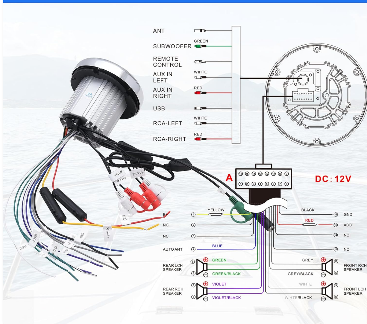
Image: Comprehensive wiring diagram illustrating all necessary connections for the Geloo Marine Stereo Receiver, including power, audio inputs/outputs, and speaker connections.
