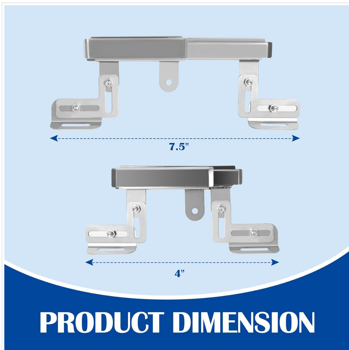
Image: Diagram illustrating the adjustable length of the crossover burner, showing approximate dimensions of 7.5 inches (extended) and 4 inches (retracted).
