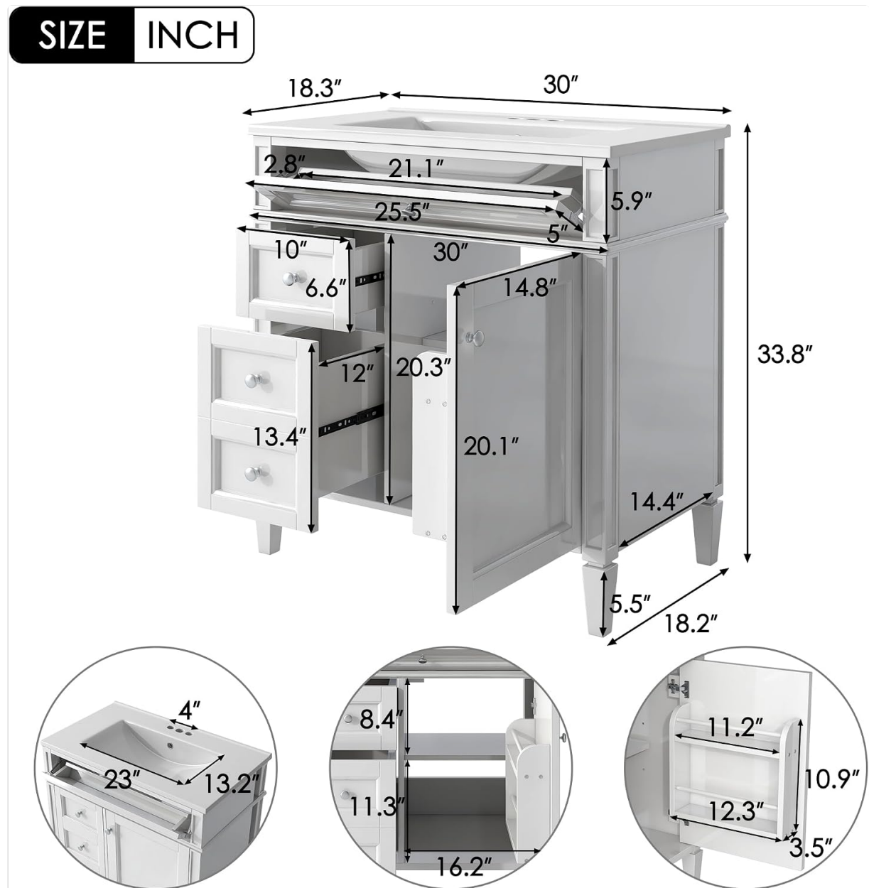
Image: Detailed dimensions of the Polibi 30-inch bathroom vanity, showing measurements for width, depth, and height, as well as internal drawer and cabinet dimensions.
