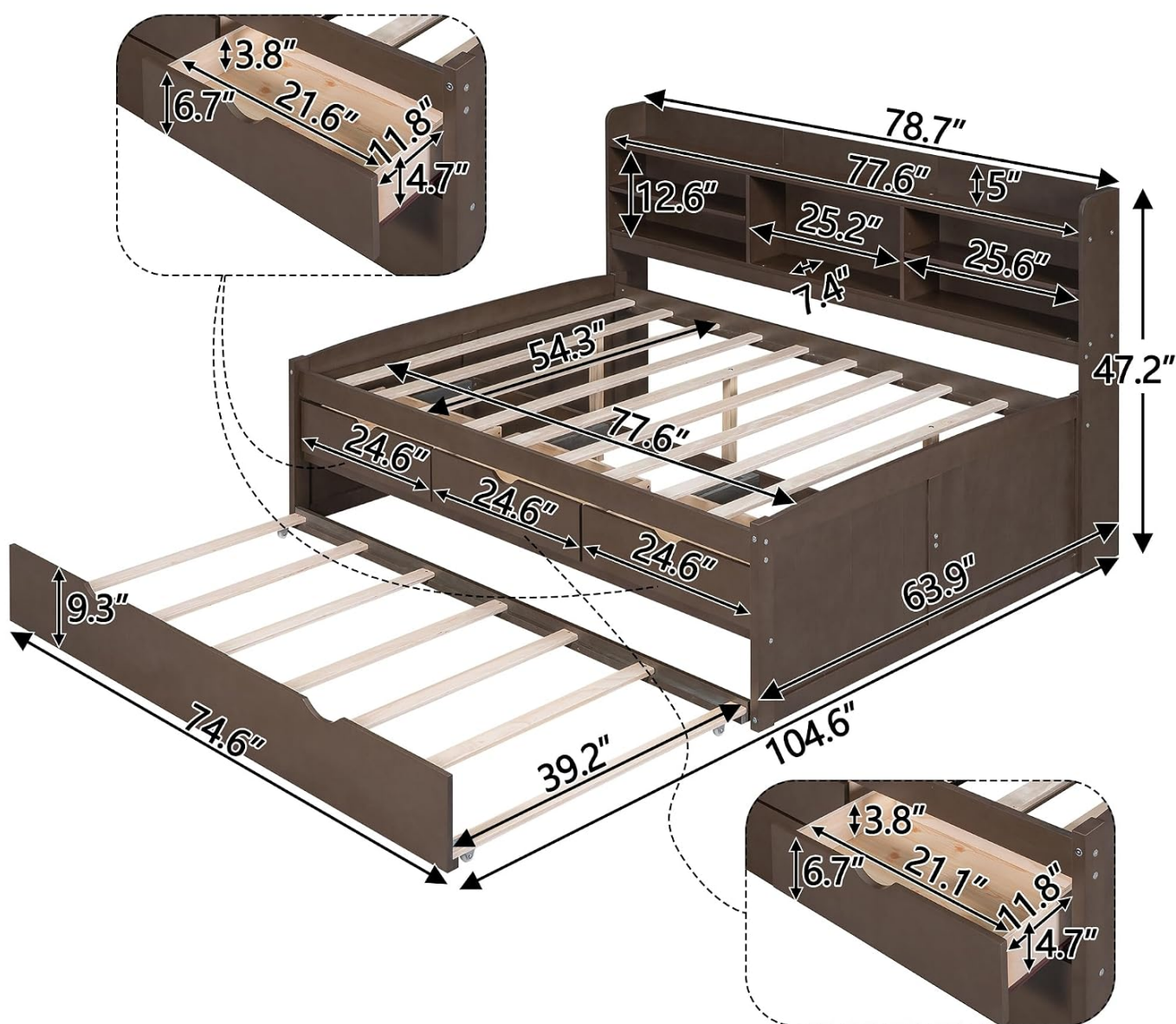
Image: Detailed dimensions of the Bellemave Full Size Captain Bed, including the main bed, trundle, and bookcase headboard. This diagram helps in identifying components and understanding the overall structure during assembly.
