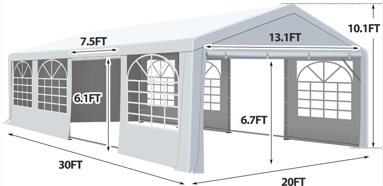
Figure 7: Tent dimensions and specifications.
