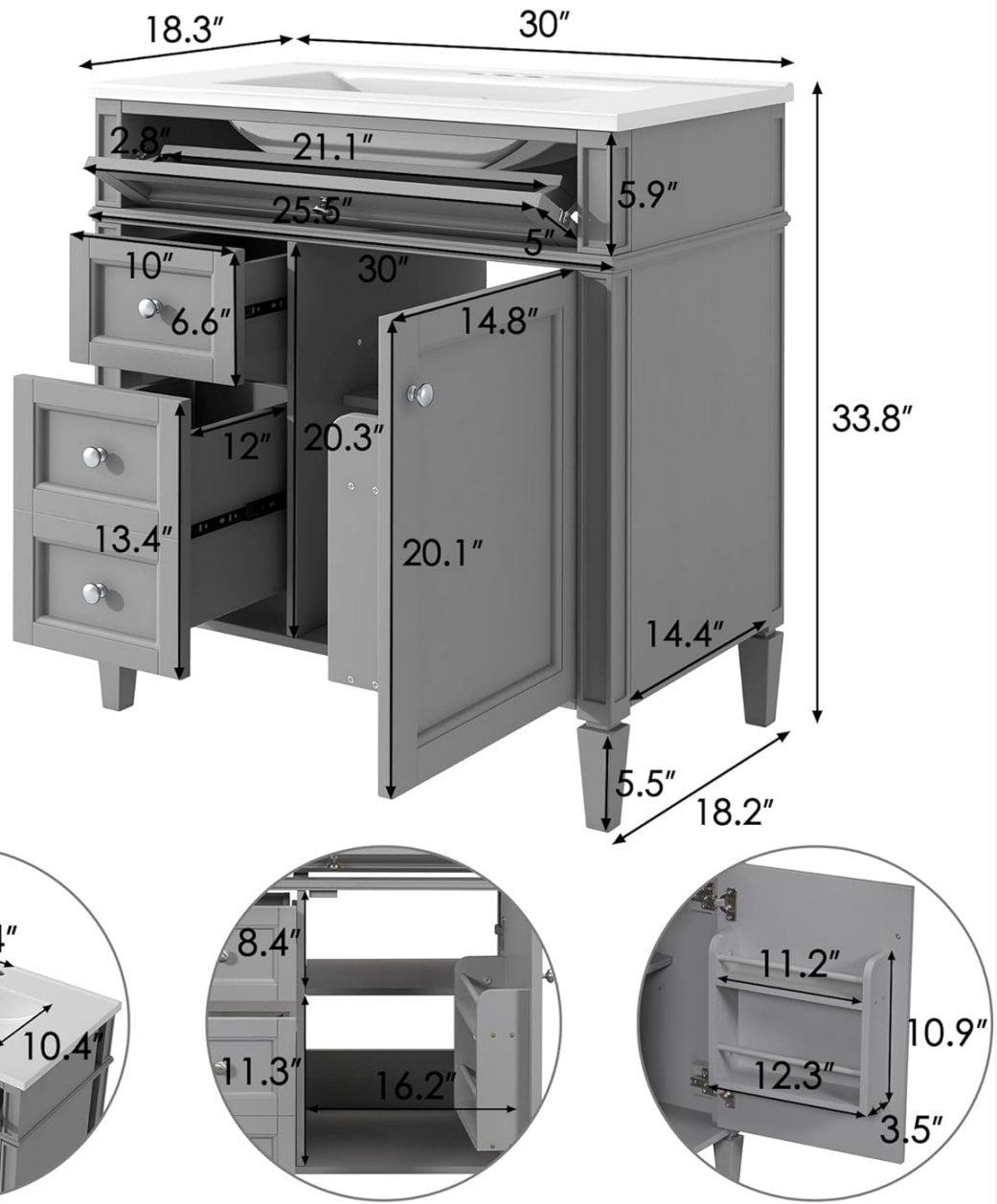
Image: A technical diagram illustrating the precise dimensions of the Virubi 30 Inch Bathroom Vanity, including width, depth, height, and internal measurements for drawers and cabinet space.
