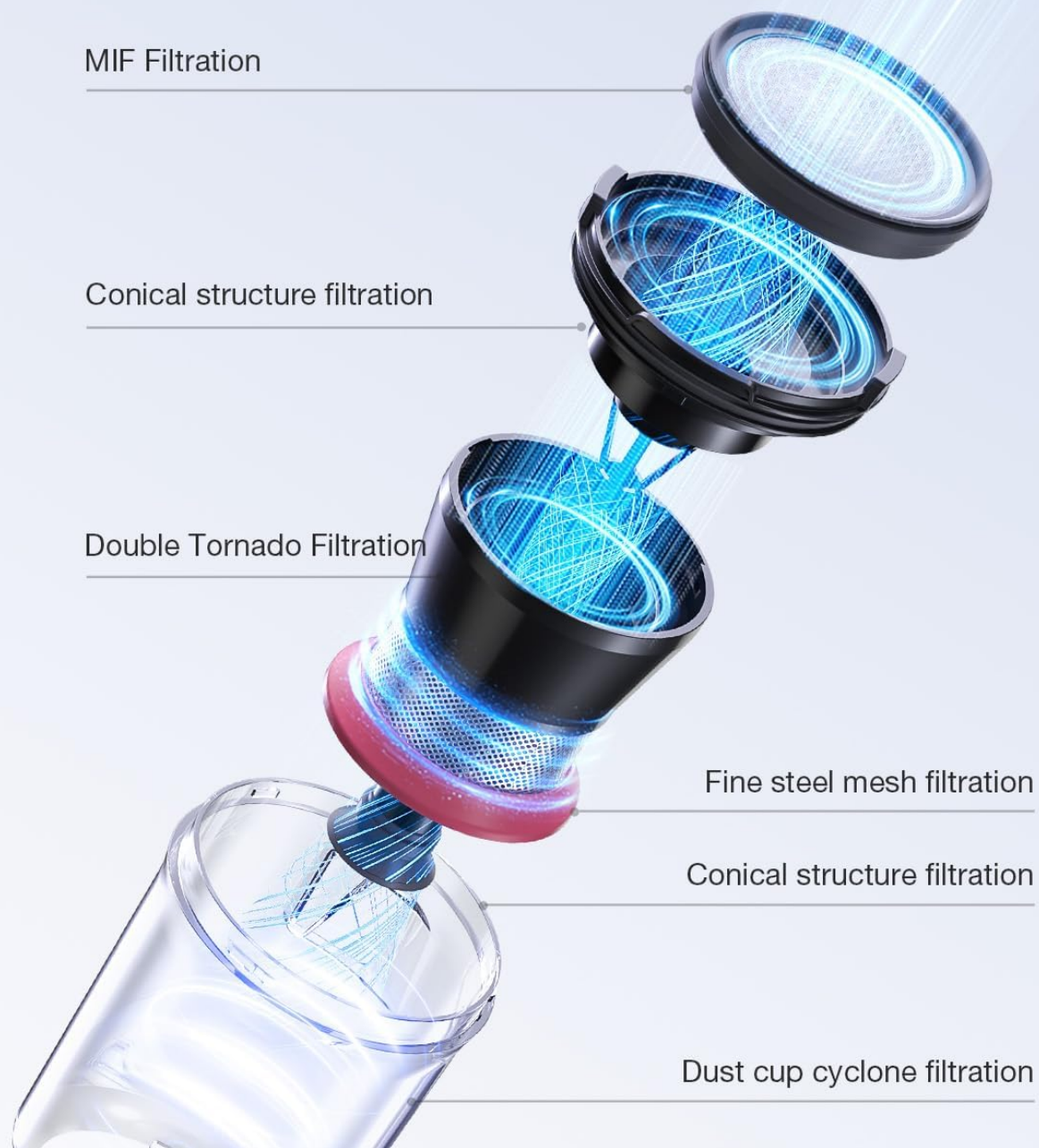
Figure 4.5: Exploded view illustrating the multi-layer dual cyclone filtration system, including MIF, conical, double tornado, and fine steel mesh filters, designed to prevent clogging and ensure long-lasting suction.
