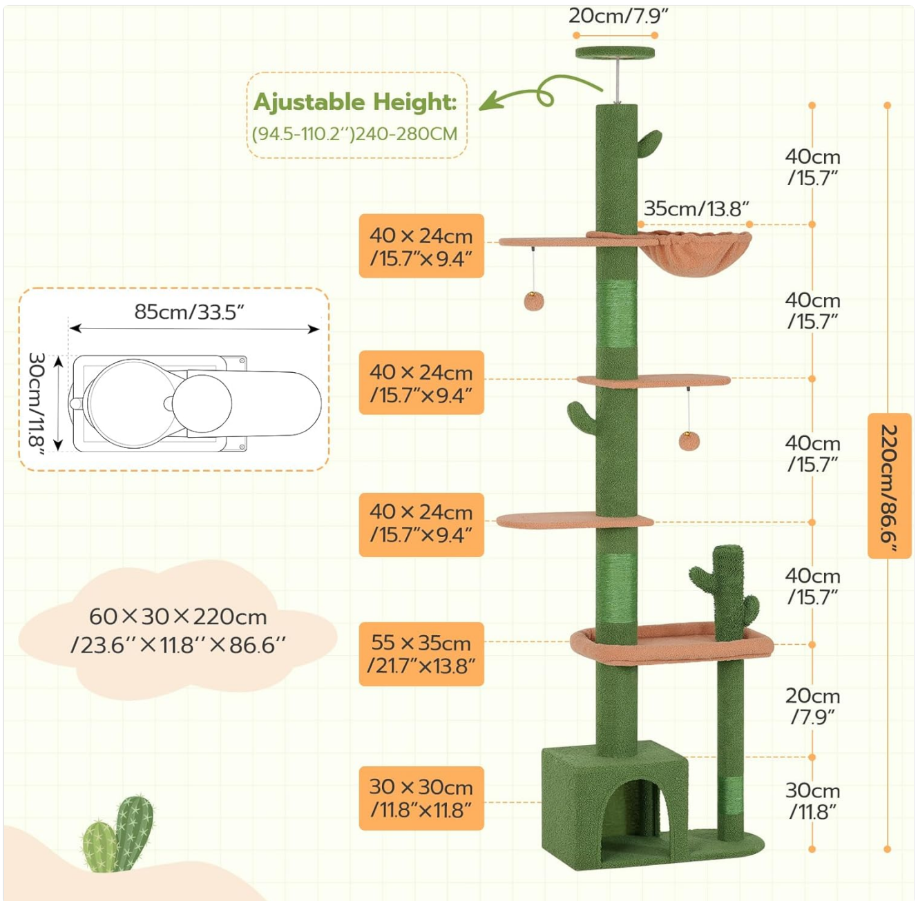
Image 2.1: Diagram illustrating the dimensions and various components of the HOOBRO Cat Tree, including platform sizes and overall height.
