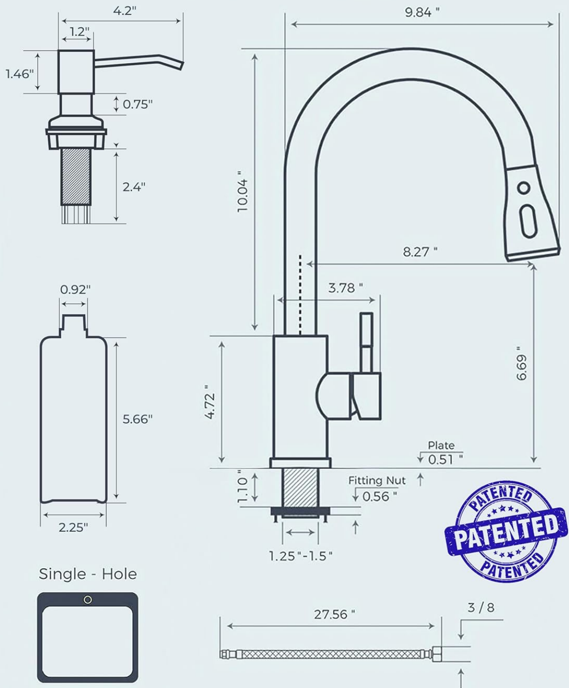
Image: Detailed diagram showing the dimensions of the faucet and soap dispenser, along with single-hole installation.
