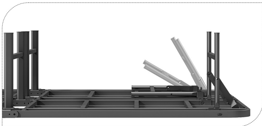
Image 5.2: The bed frame in its folded configuration.
