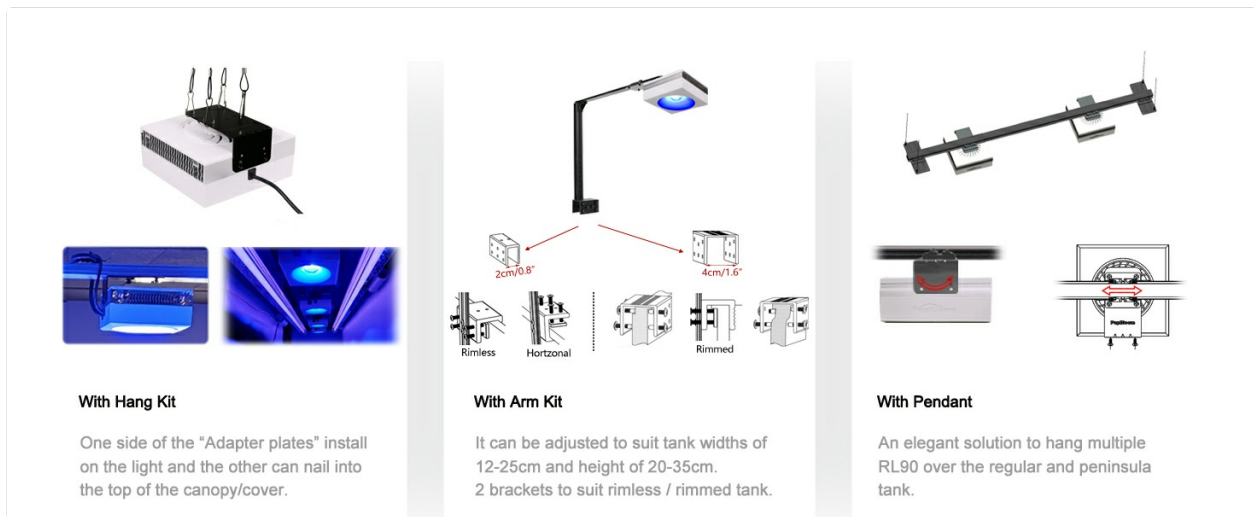
Figure 4.2: Mounting Options (Hang Kit, Arm Kit, Pendant)
