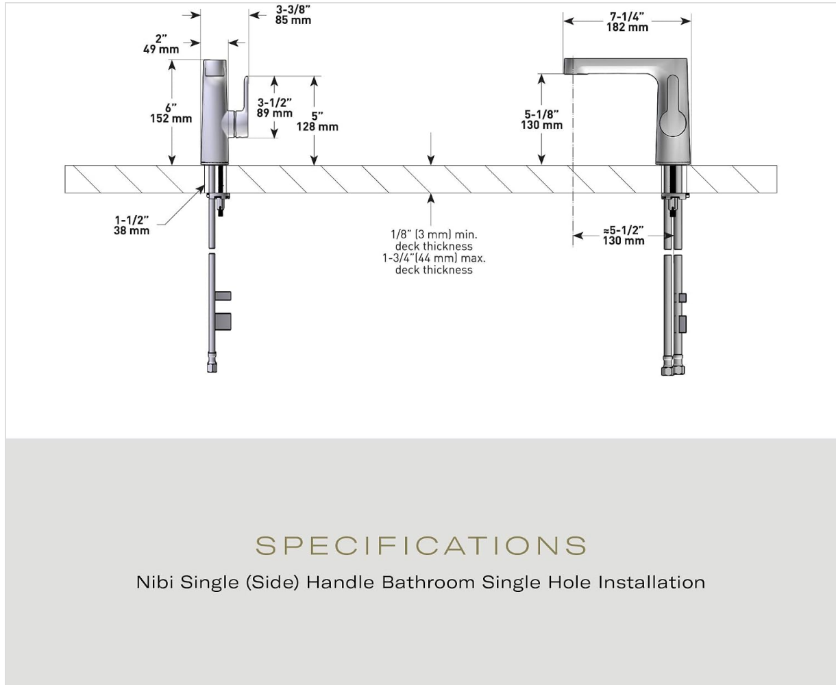
Image 4.1: Key dimensions for the Riobel Nibi Single Hole Bathroom Faucet, including spout reach and overall height.
