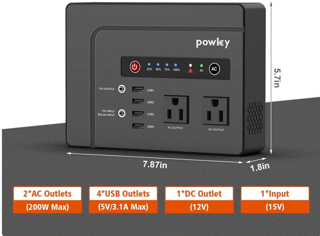
Image: Close-up view of the powkey HP200 power station, highlighting its 2 AC outlets, 4 USB outlets, 1 DC outlet, and 1 input port, along with its compact dimensions.
